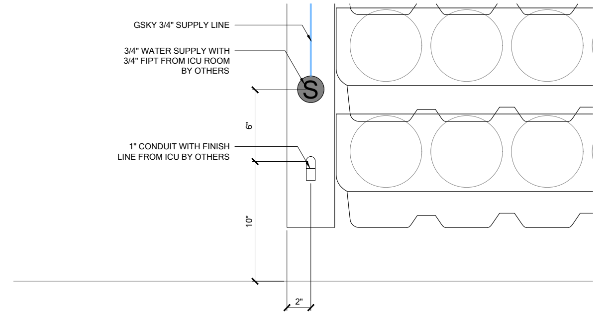
3 ELEVATION DETAIL SCALE 1 1/2" = 1'-0"
