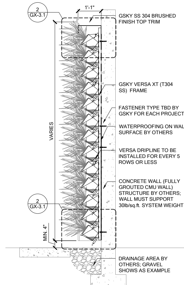
3 SECTION SCALE 3/8" = 1'-0"
