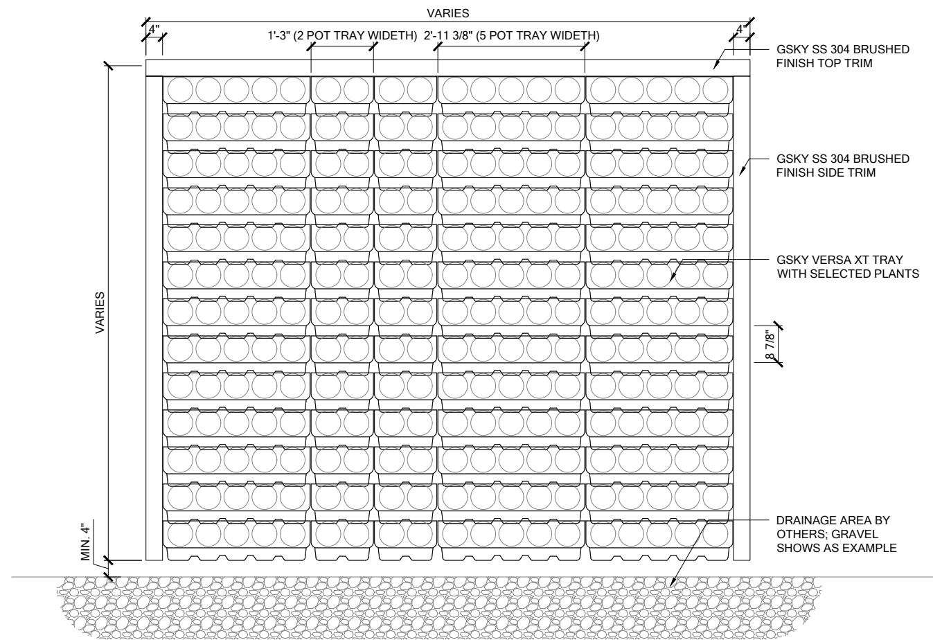
1 ELEVATION SCALE 3/8" = 1'-0"
