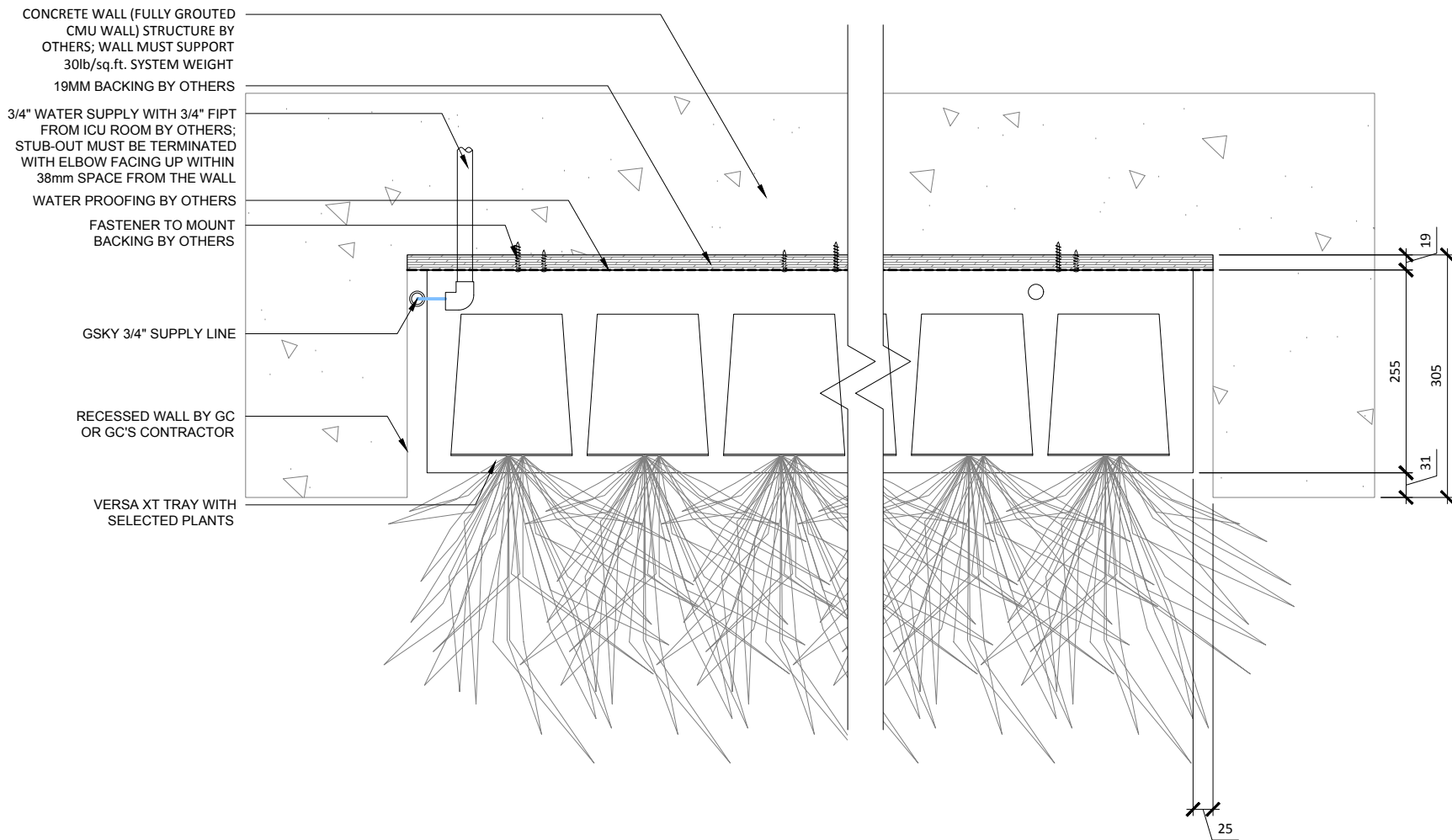
1 PLAN DETAIL SCALE: 1:8
