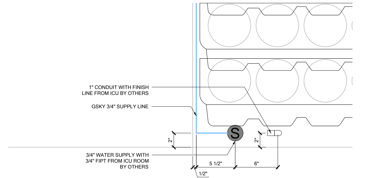
3 ELEVATION DETAIL SCALE 1 1/2" = 1'-0"
