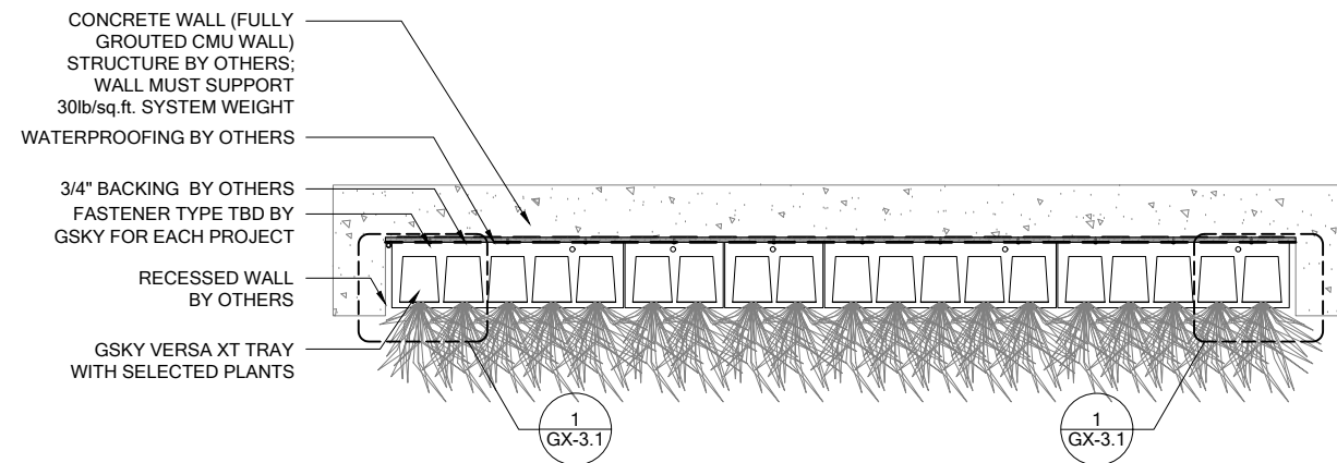
2 PLAN SCALE 3/8" = 1'-0"
