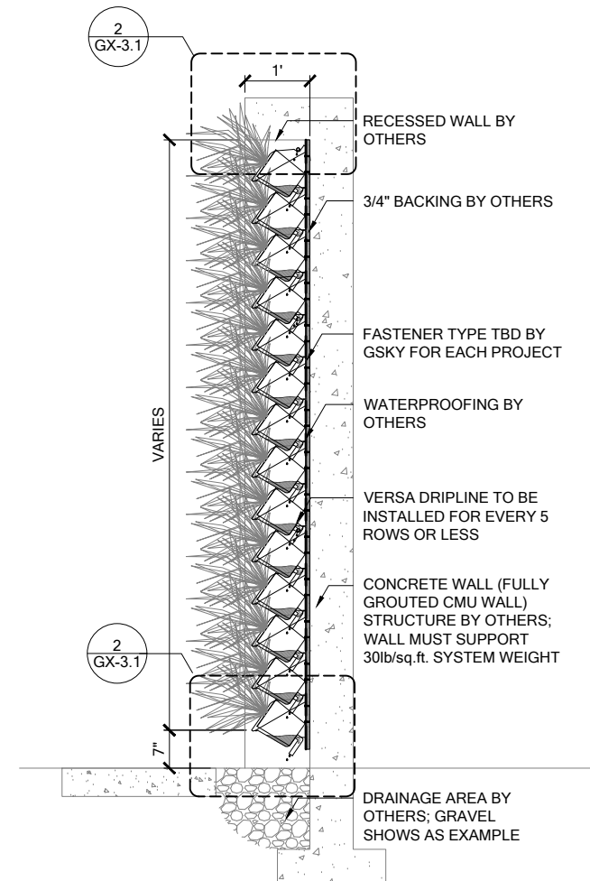
3 SECTION SCALE 3/8" = 1'-0"
