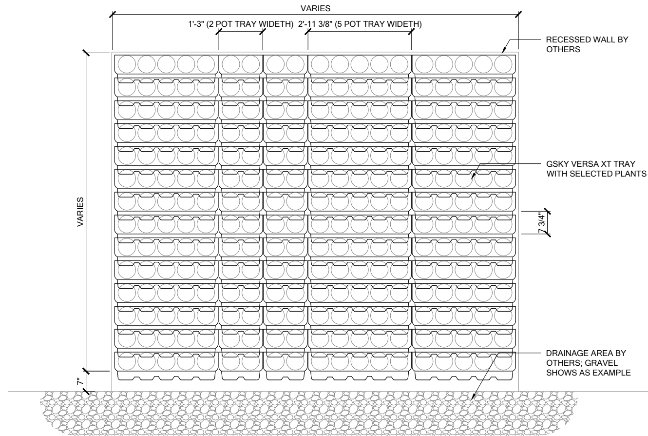
1 ELEVATION SCALE 3/8" = 1'-0"
