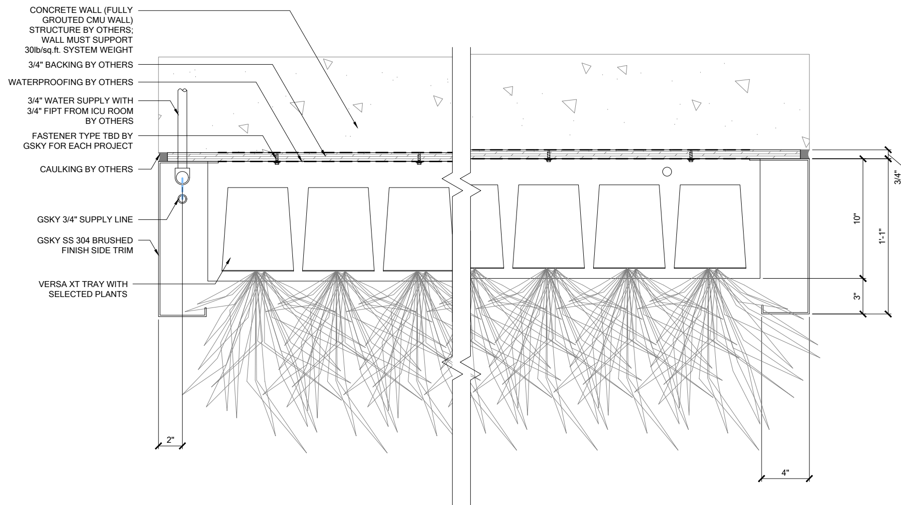
1 PLAN DETAIL SCALE 1 1/2" = 1'-0"
