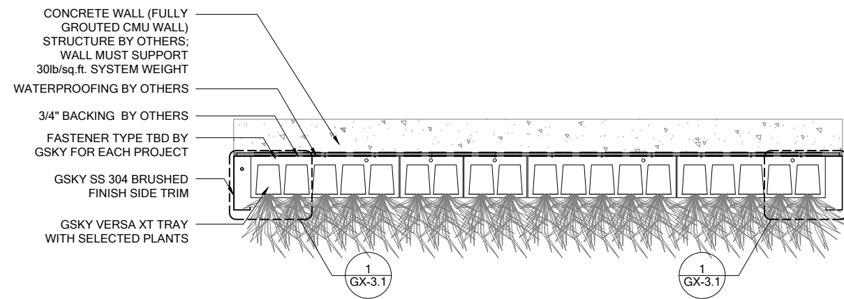
2 PLAN SCALE 3/8" = 1'-0"
