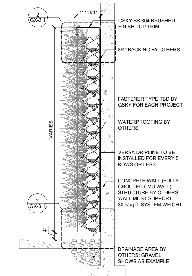
3 SECTION SCALE 3/8" = 1'-0"
