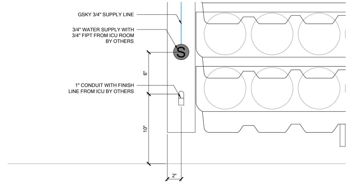
3 ELEVATION DETAIL SCALE 1 1/2" = 1'-0"
