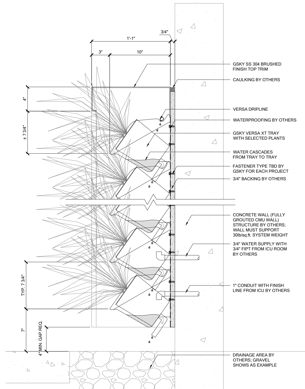
2 SECTION DETAIL SCALE 1 1/2" = 1'-0"
