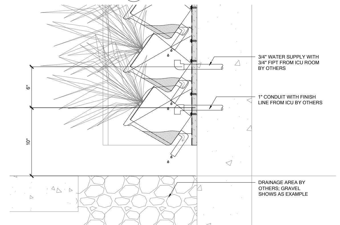
2 SECTION SCALE 1 1/2" = 1'-0"
