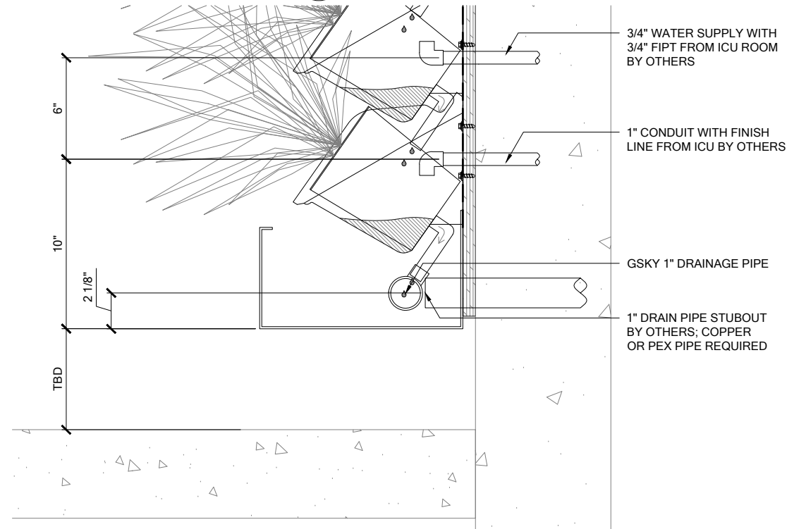
2 SECTION SCALE 1/2" = 1'-0"
