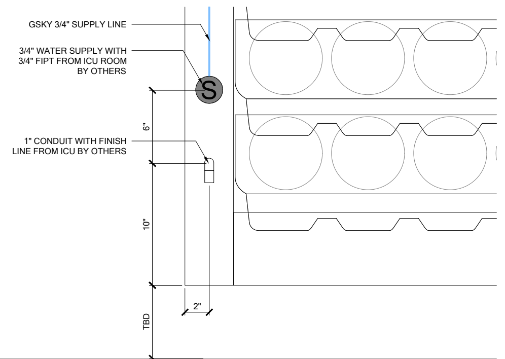
3 ELEVATION DETAIL SCALE 1/2" = 1'-0"
