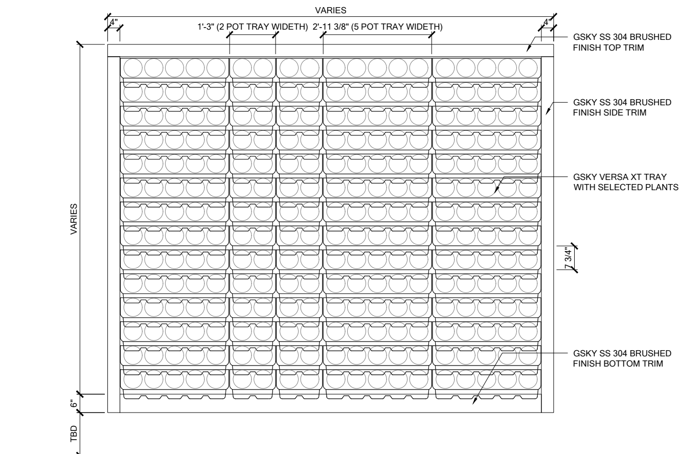
1 ELEVATION SCALE 3/8" = 1'-0"
