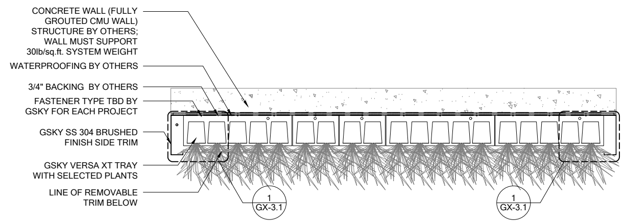
2 PLAN SCALE 3/8" = 1'-0"
