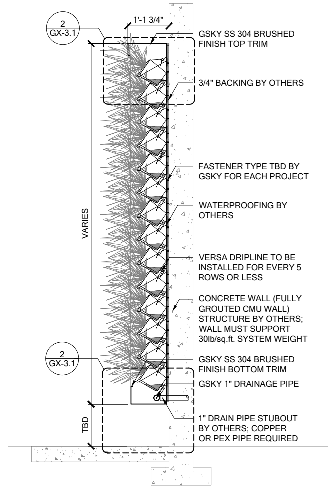
3 SECTION SCALE 3/8" = 1'-0"
