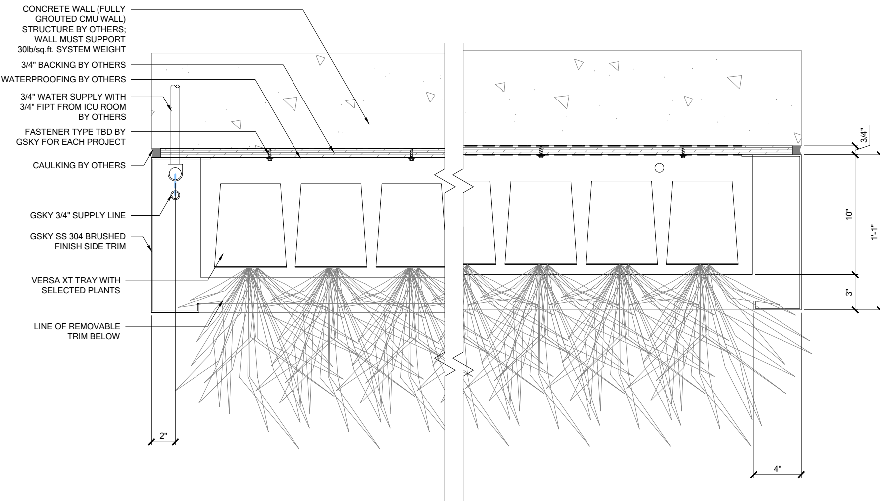
1 PLAN DETAIL SCALE 1 1/2" = 1'-0"
