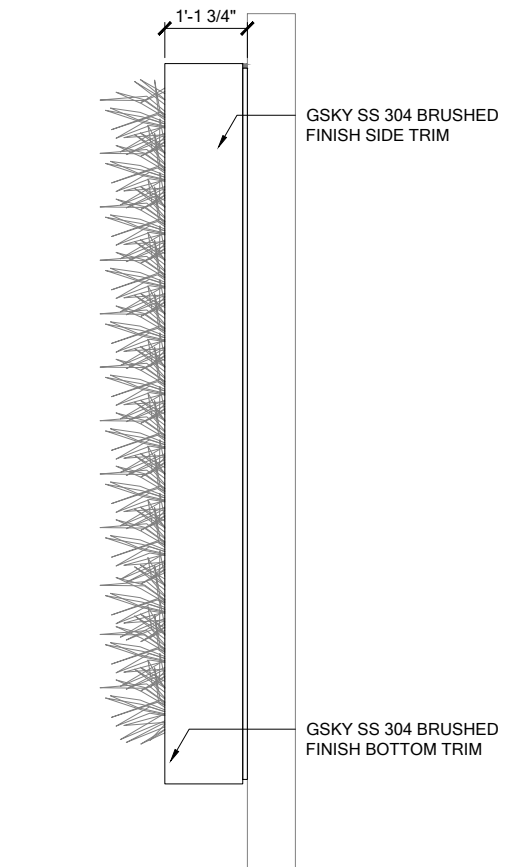
4 SIDE SCALE 3/8" = 1'-0"
