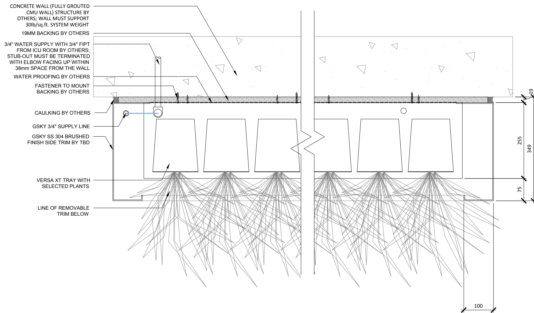
1 PLAN DETAIL SCALE: 1:8
