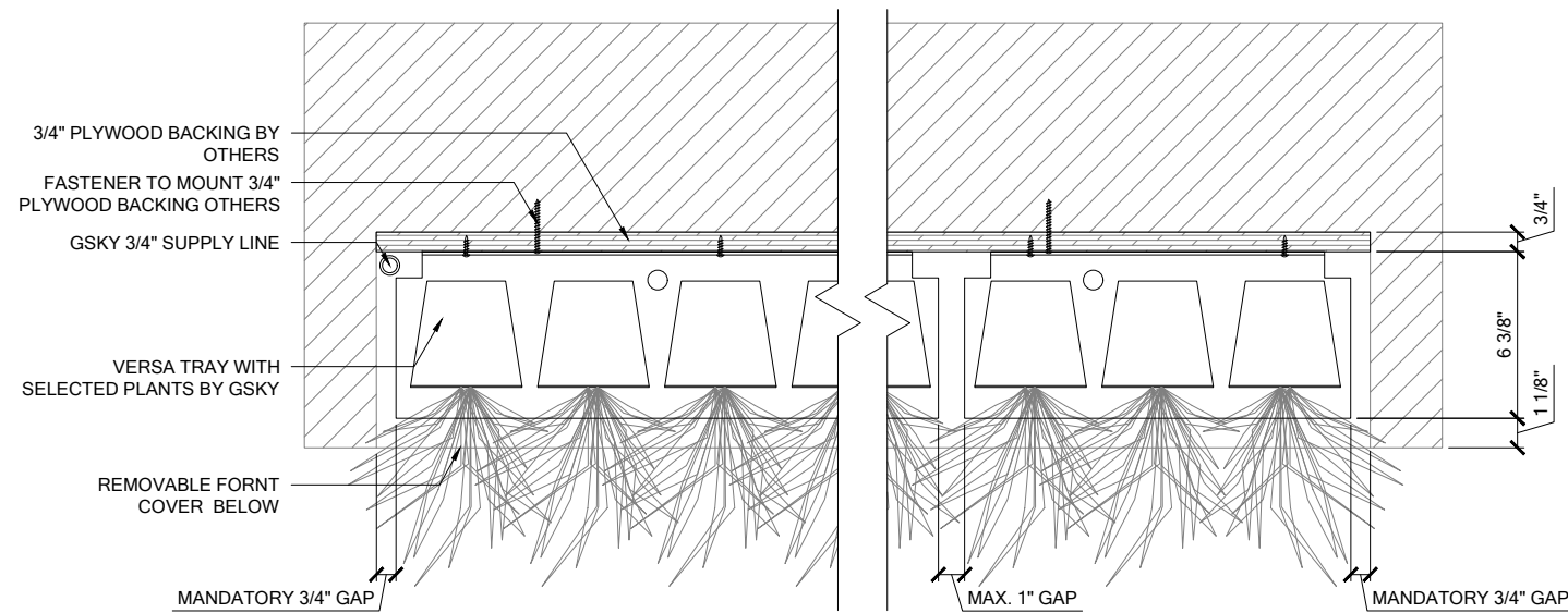
1 PLAN SCALE 1 1/2" = 1'-0"
