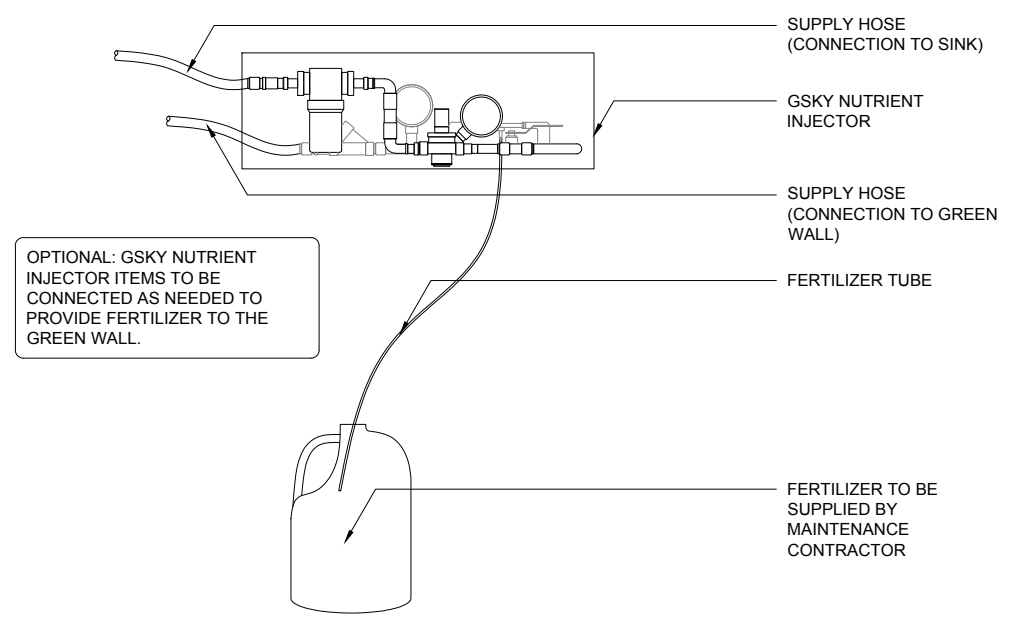
2 OPTIONAL: GSKY NUTRIENT INJECTOR SCALE 1" = 1'-0"
