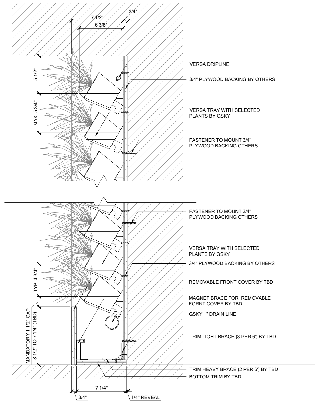
2 SECTION SCALE 1 1/2" = 1'-0"
