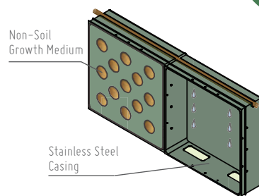
Green Wall Panel Detail
